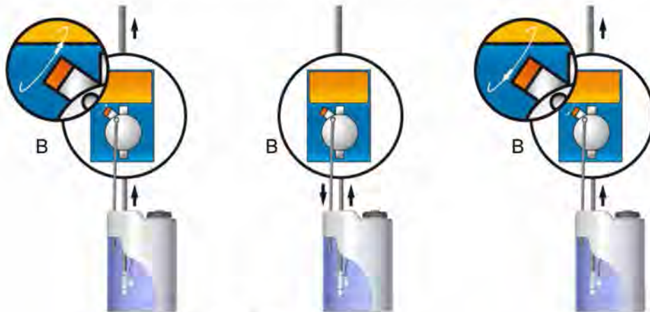
Fig.5 – Priming sequence
