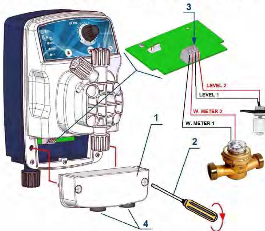
Fig. 9 – Level probe and water meter connection
