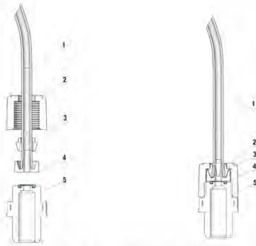
Fig.4 – Tubes connection
