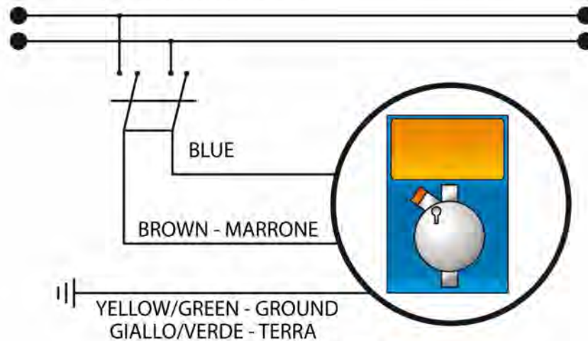
Fig.3 - Electrical Scheme
