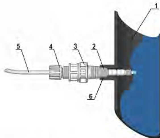
Fig. 7 – Injection valve installation
